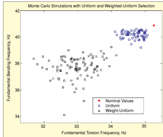
Figure 17. Second robustness study – scatter of fundamental eigenfrequency values as a result of breaking a subset of spot welds with a weighted-uniform selection probability. For comparison, the results of the first robustness study in Figure 16 are also shown.
