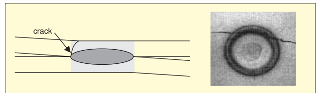
Figure 5. A typical sheet fracture fatigue crack (left) and a photo of the crack propagation along the surface of the base sheet material (right).
