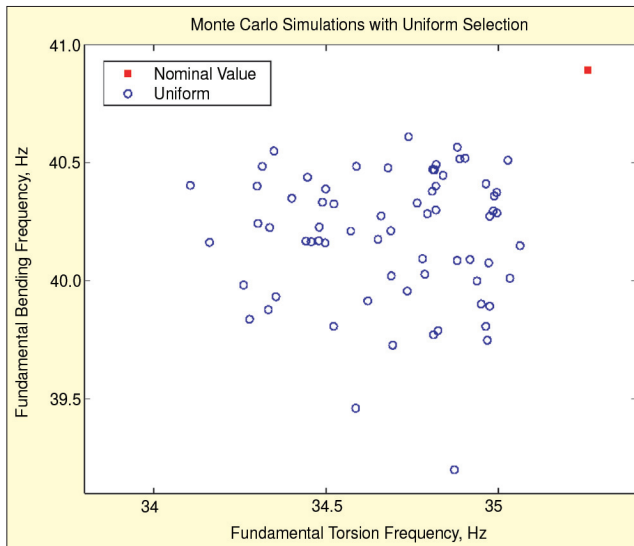
Figure 16. First robustness study – scatter of fundamental eigenfrequency values as a result of breaking a subset of spot welds with a uniform selection probability.
