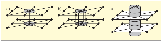
Figure 6. The spot weld models investigated in Reference 13.
