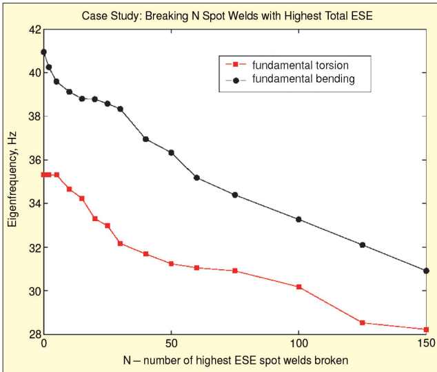
Figure 15. The effect of breaking a subset of spot welds with highest total ESE at the fundamental torsion and bending eigenfrequency.
