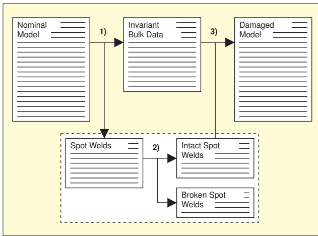
Figure 12. File management procedures – from the nominal vehicle model, a damaged model is generated, with a number of broken spot weld connections.
