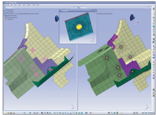
Figure 11. LMS Virtual.Lab spot weld modeling for durability. For the analysis step, a coarse spot weld connection is used (the HEXA model, left) to identify the most critical spot welds. For the second analysis step, the critical spot welds are replaced by a more detailed spot weld model (right) to allow more accurate local stress predictions.
