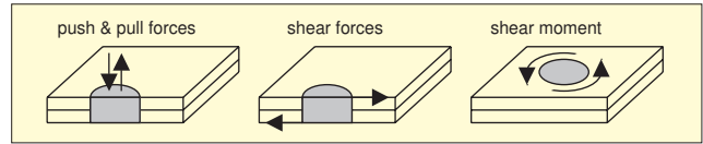
Figure 4. Forces and moments that can be transmitted by a spot weld.
