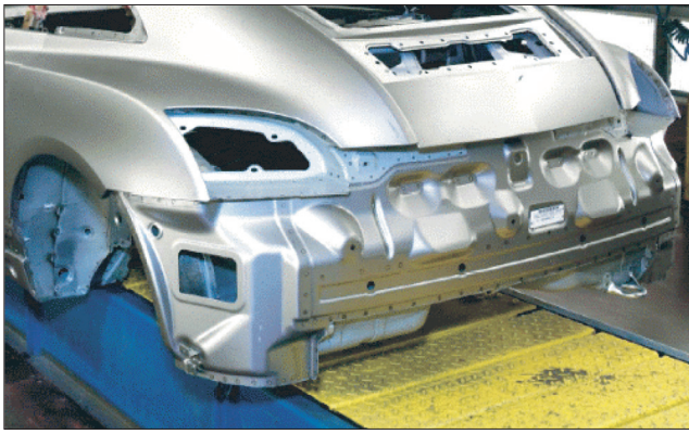
Figure 1. A spot-welded vehicle body-in-white. 1
