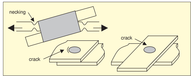
Figure 3. Failure mechanism for lap-shear sample (left) and cross-tension sample (right).
