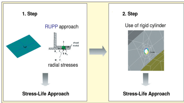
Figure 10. Two-step approach for spot weld fatigue life prediction.
