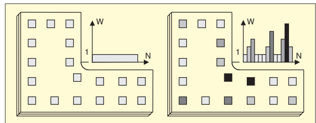
Figure 13. Random selection schemes – uniform selection procedure for all N spot welds (left), and a weighted-uniform selection probability, using an integer weighting factor W (right).
