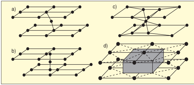
Figure 7. The four spot weld models investigated for NVH predictions in Reference 5.
