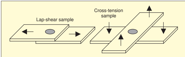
Figure 2. Lap-shear and cross-tension geometry.
