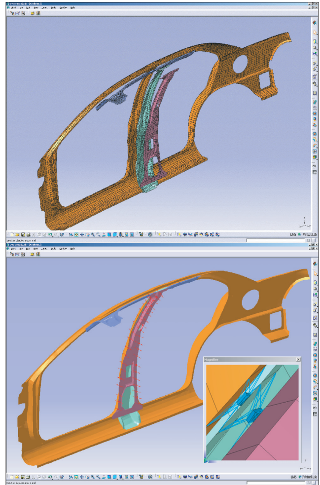
Figure 8. LMS Virtual.Lab spot weld modeling for NVH – B-pillar connection. Four panels are to be connected (top). First, the spot weld locations are defined (bottom). At these locations, HEXA spot welds are then created (insert, bottom right – a magnification of 2 HEXA spot welds).
