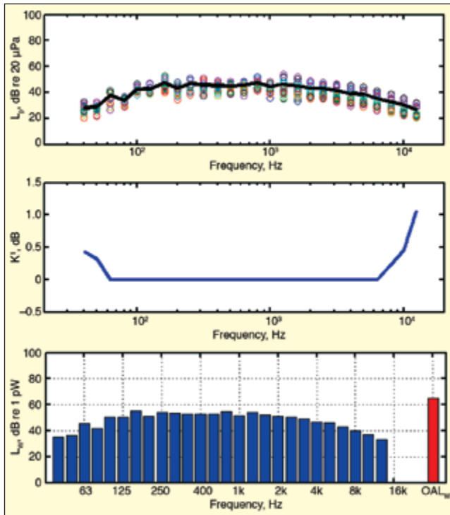
Figure 6. Sound power measurement results – dehumidifier.
