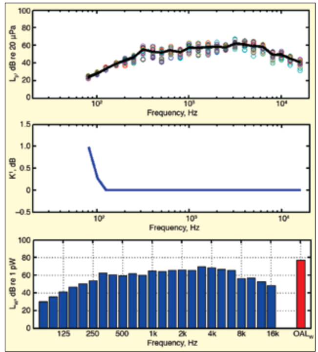
Figure 7. Sound power measurement results – cordless electric vacuum.
