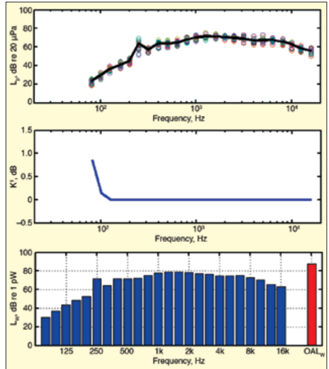
Figure 8. Sound power measurement results – blender/mixer.
