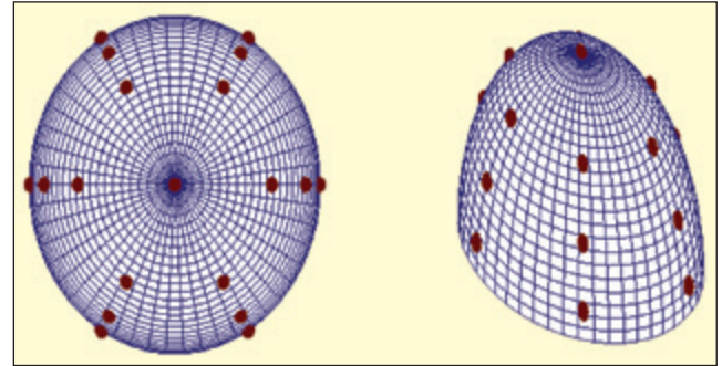
Figure 4. Schematic of 20 hemispherical microphone locations (red dots) specified in Annex B of ANSI-ASA S12.54/ISO 3744 shown from top view (left) and isometric view (right).
