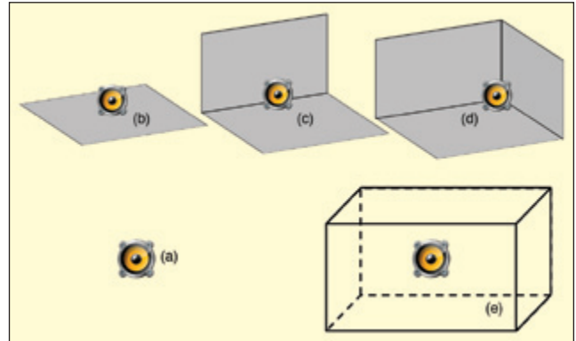
Figure 2. Examples of environments for sound power measurements: (a) free field; (b) free field over one reflecting plane; (c) free field over two reflecting planes; (d) free field over three reflecting planes; and (e) reverberant field.
