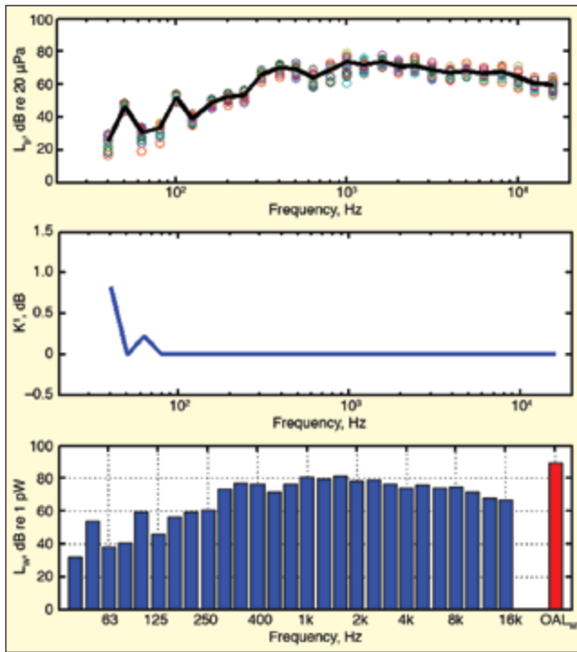
Figure 5. Sound power measurement results – 100-psi air compressor.
