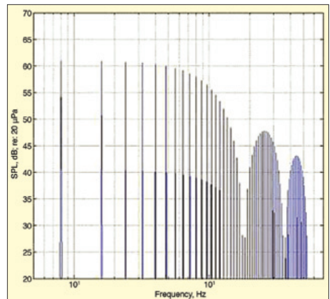
Figure 14. Spectrum of \sin(x)/x -weighted BPF harmonics.
