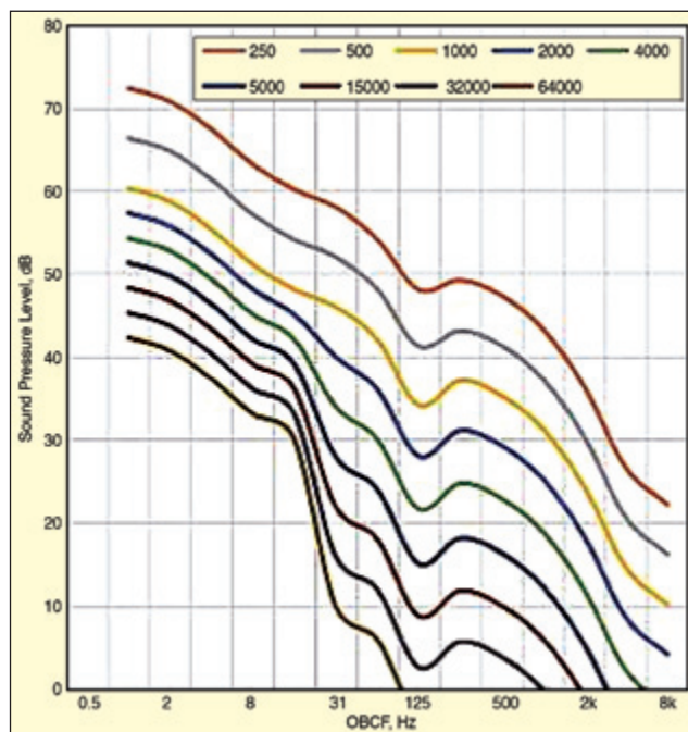
Figure 18. Calculated L_p spectra as function of distance.
