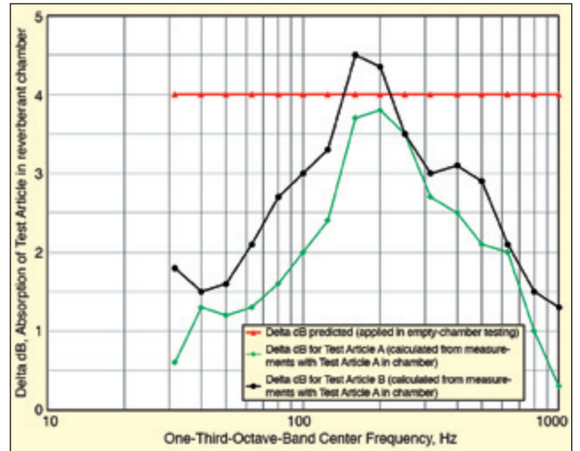
Figure 2. Illustration of delta SPL dB for two notional test articles.
