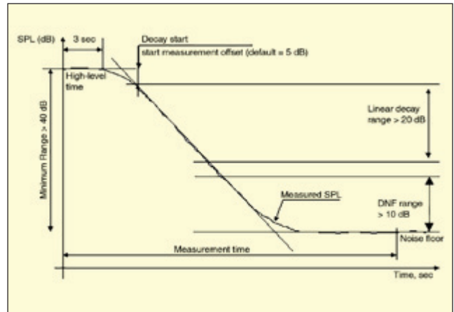
Figure 1. ISO354 Interrupted Noise Method of determining reverberant room decay rates.
